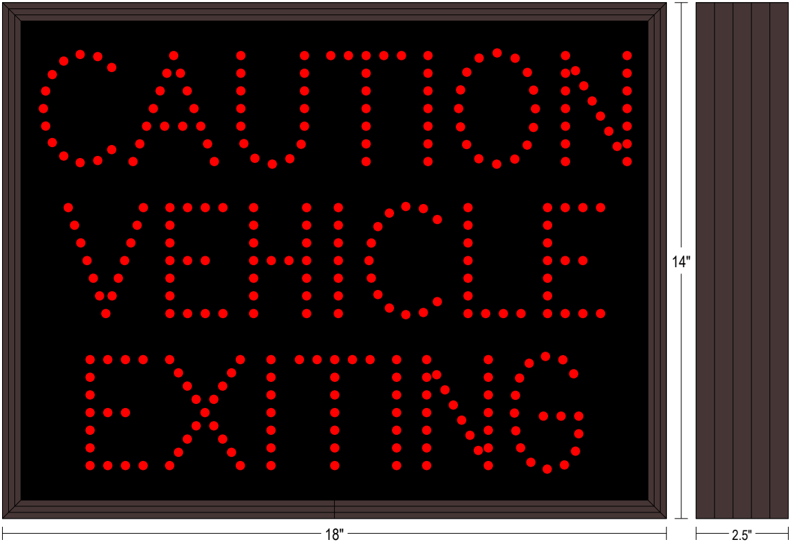
Frame Detail
