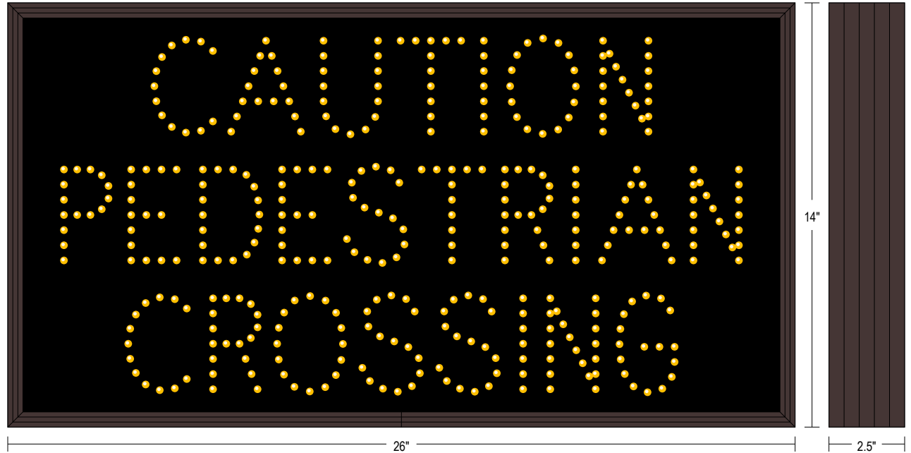
Frame Detail
