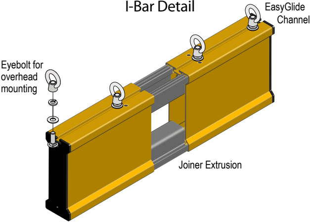
I-Bar Detail
