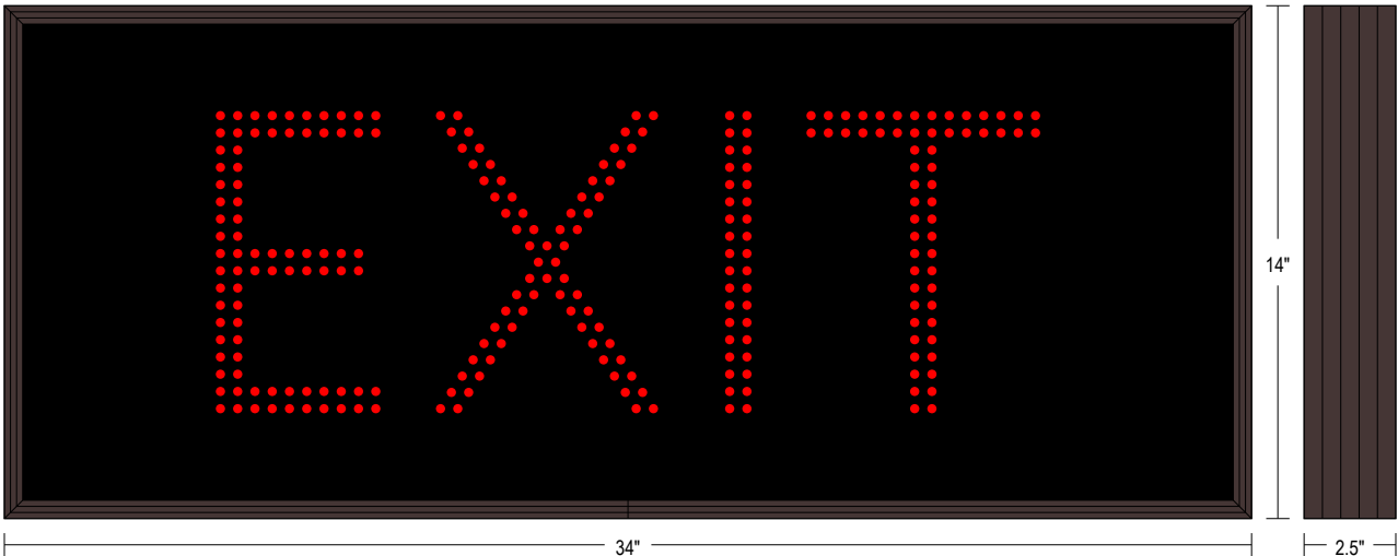
Frame Detail
