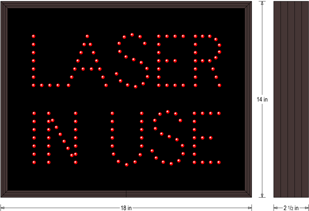
Frame Detail
