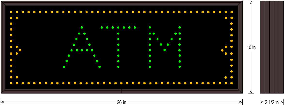
Frame Detail
