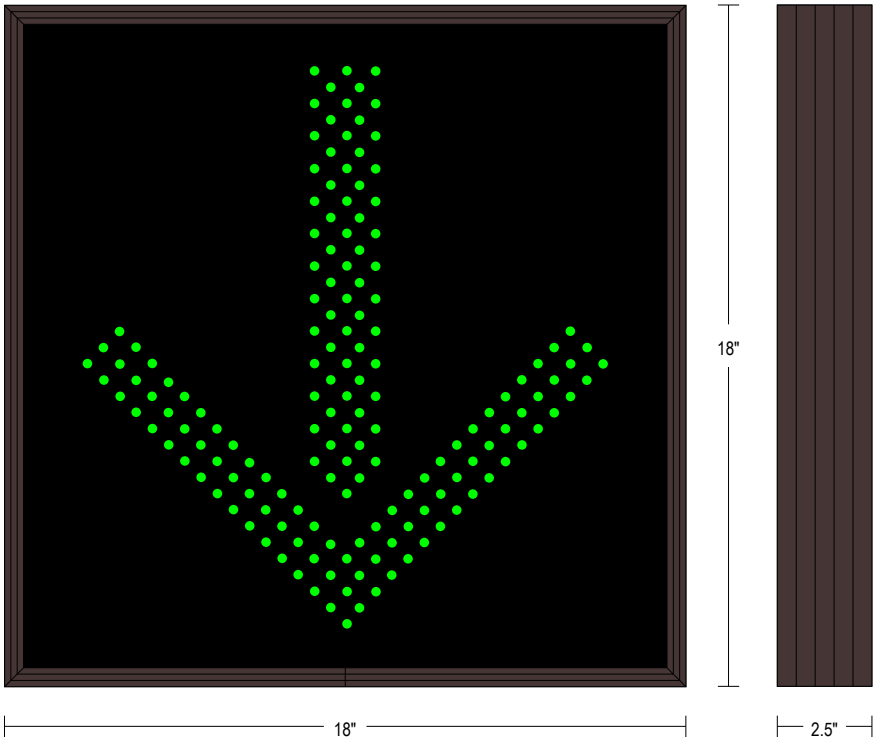
Frame Detail
