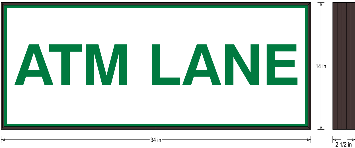
Frame Detail
