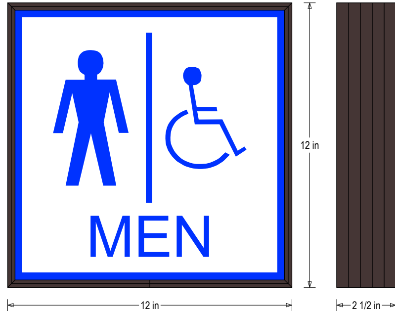
Frame Detail
