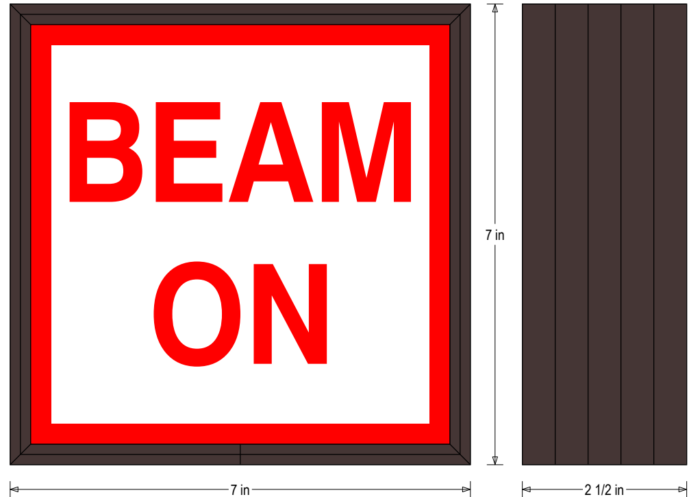
Frame Detail
