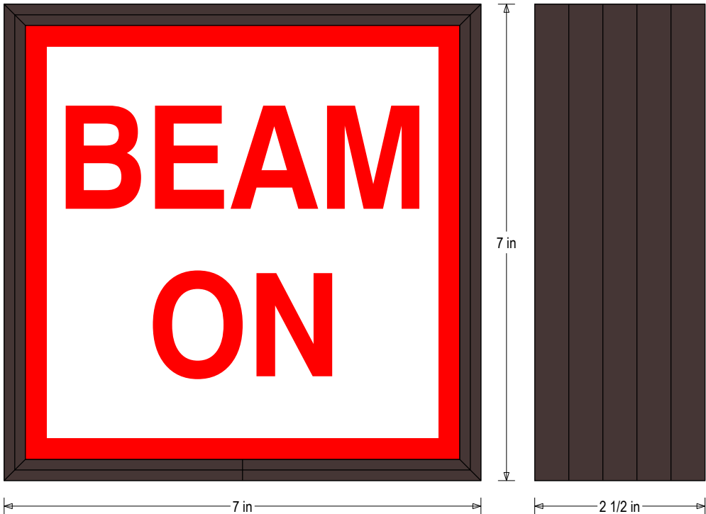
Frame Detail
