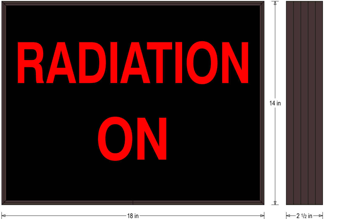
Frame Detail
