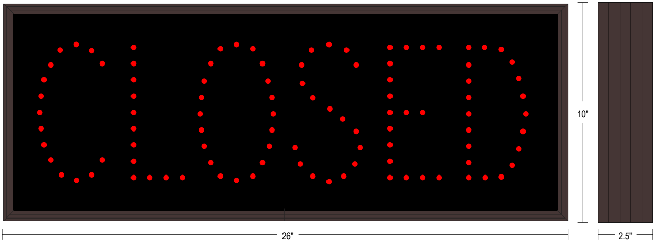
Frame Detail
