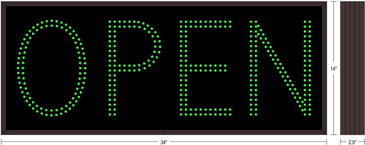
Frame Detail
