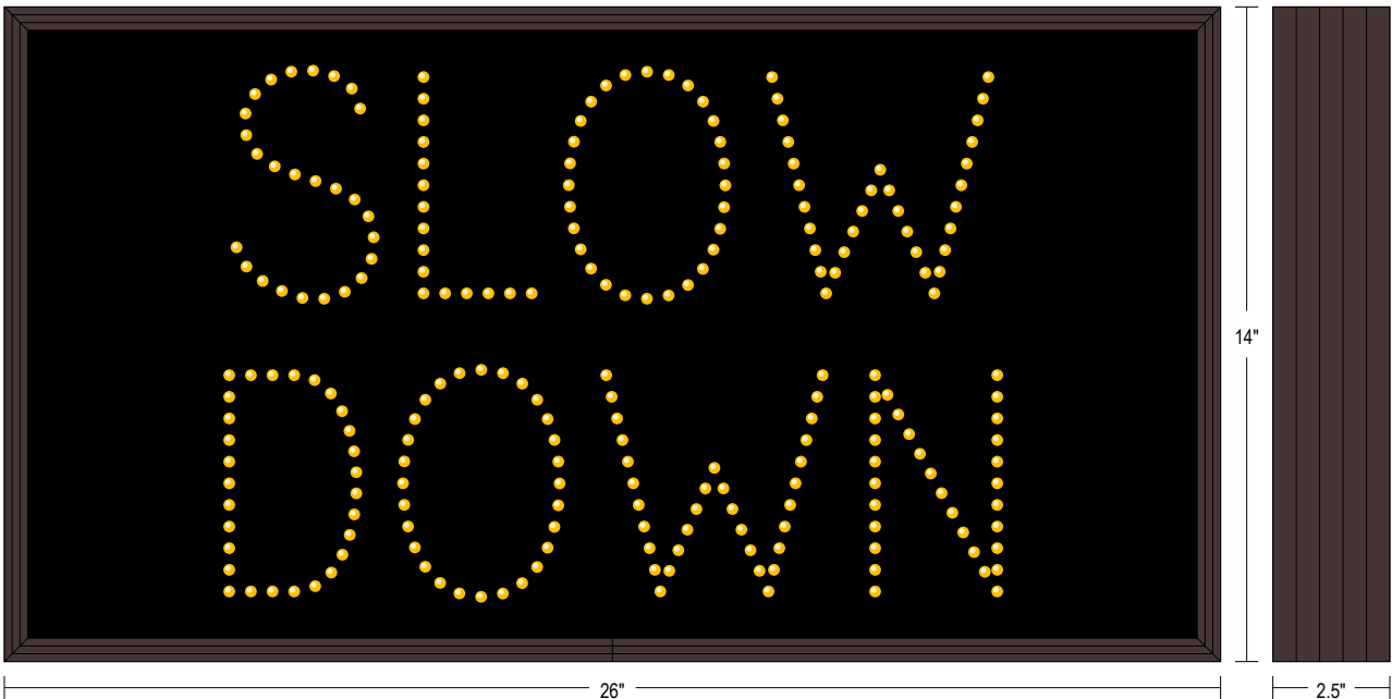
Frame Detail
