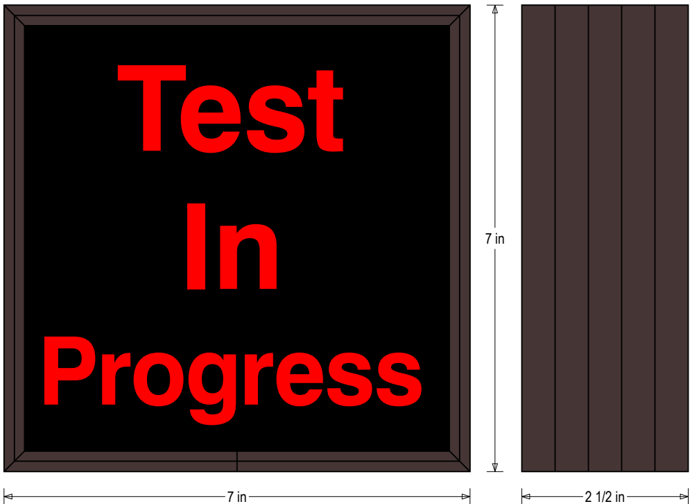
Frame Detail
