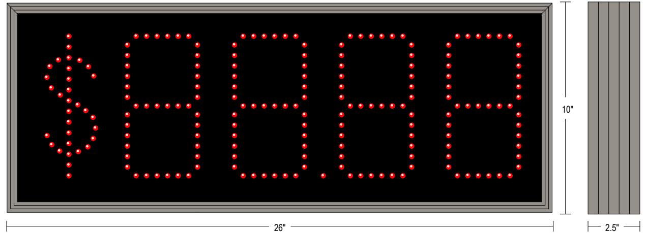
FRONT VIEW
