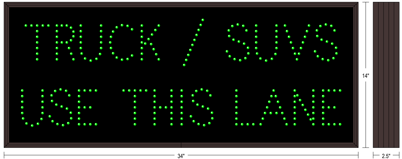
Frame Detail
