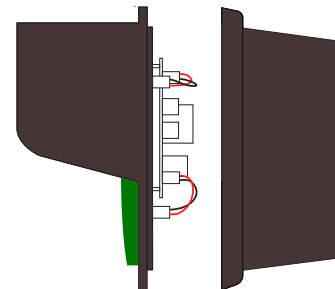
Replaceable Circuit Board Assembly
