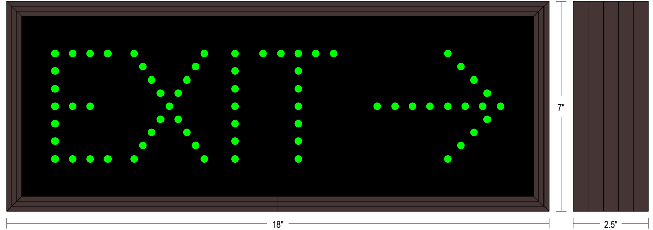
Frame Detail
