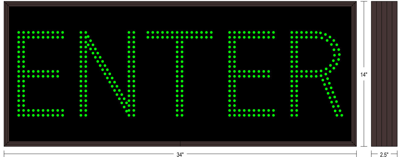
Frame Detail
